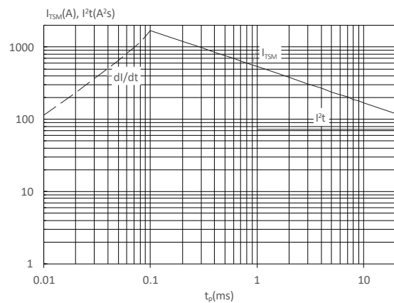
FIG : Non-repetitive surge peak on-state current for a sinusoidal pulse with width t_p < 20ms , and corresponding value of I^2t ( dl/dt < 100A/\mu s )
