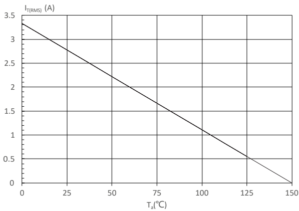
FIG : On-state characteristics
