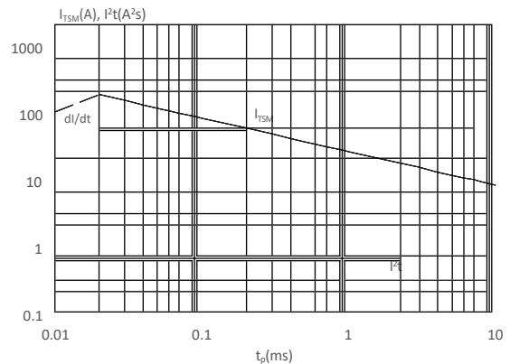
FIG : Non-repetitive surge peak on-state current for a sinusoidal pulse with width t_p < 10\text{ms} , and corresponding value of I^2t ( di/dt < 50\text{A}/\mu\text{s} )
