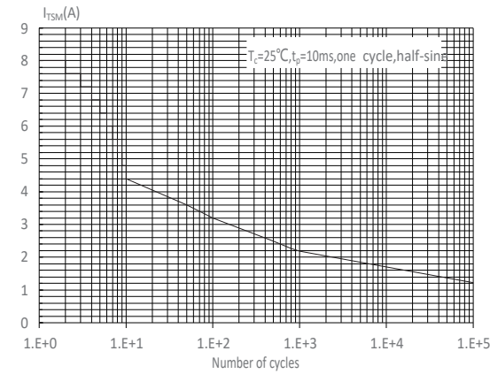
FIG : Non-repetitive surge peak on-state current for a sinusoidal pulse with width t_p < 10\text{ms} , and corresponding value of I^2t ( di/dt < 50\text{A}/\mu\text{s} )
