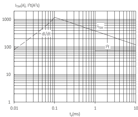
FIG : Non-repetitive surge peak on-state current for a sinusoidal pulse with width t_p < 10ms , and corresponding value of I^2t ( di/dt < 100A/\mu s )
