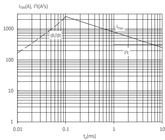
FIG : Non-repetitive surge peak on-state current for a sinusoidal pulse with width t_p < 10ms , and corresponding value of I^2t ( di/dt < 150A/\mu s )
