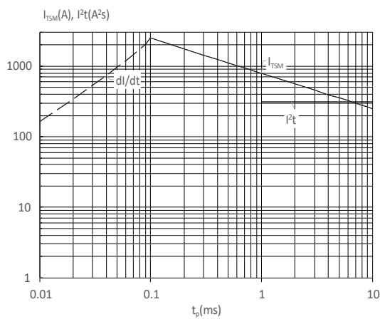
FIG : Non-repetitive surge peak on-state current for a sinusoidal pulse with width t_p < 10ms , and corresponding value of I^2t ( di/dt < 150A/\mu s )
