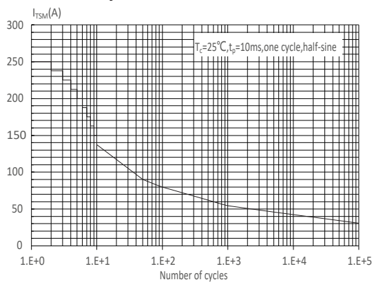
FIG : Non-repetitive surge peak on-state current for a sinusoidal pulse with width t_p < 10ms , and corresponding value of I^2t ( di/dt < 150A/\mu s )
