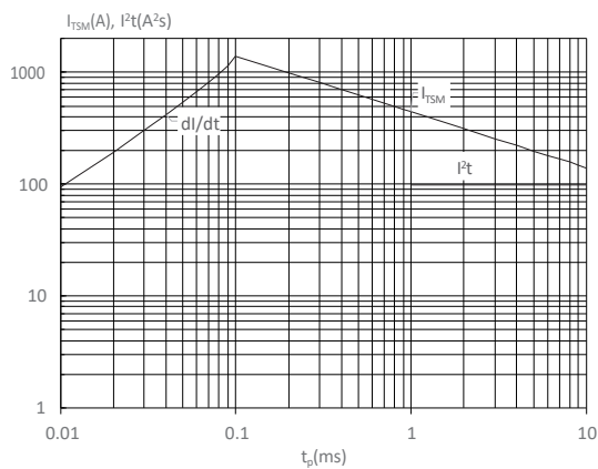
FIG : Non-repetitive surge peak on-state current for a sinusoidal pulse with width t_p < 10ms , and corresponding value of I^2t ( di/dt < 150A/\mu s )
