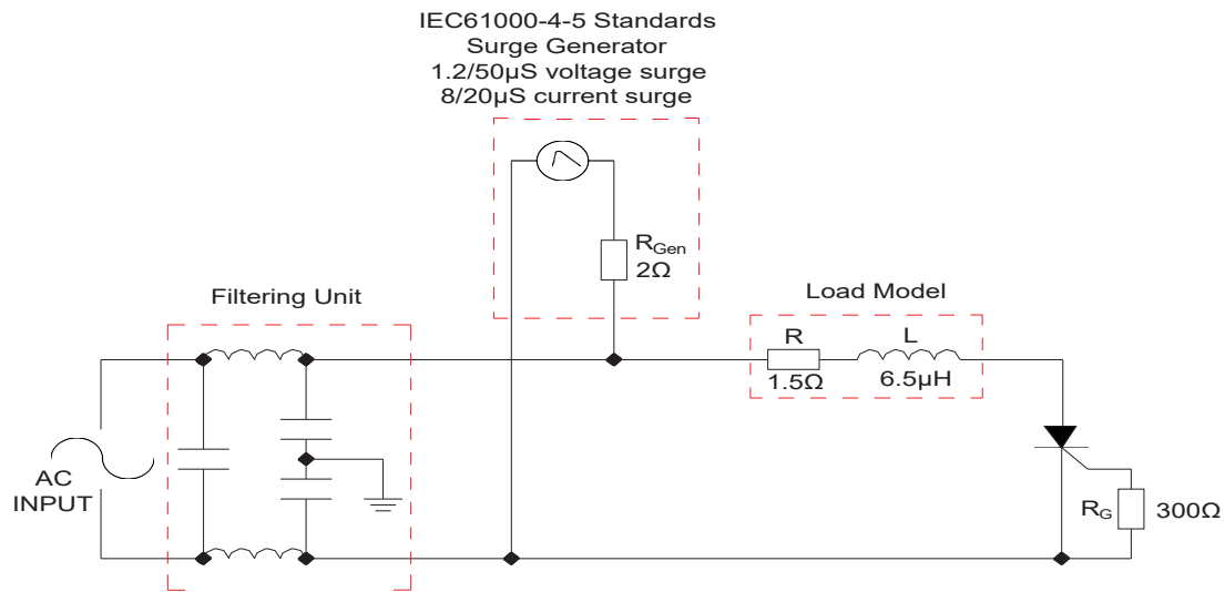
FIG : Test circuit for inductive and resistive loads to IEC-61000-4-5 standards.
