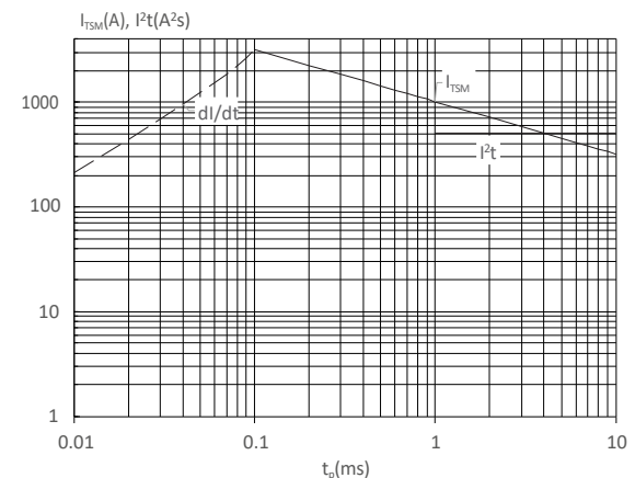
FIG : Non-repetitive surge peak on-state current for a sinusoidal pulse with width t_p < 10ms , and corresponding value of I^2t ( di/dt < 200A/μs )
