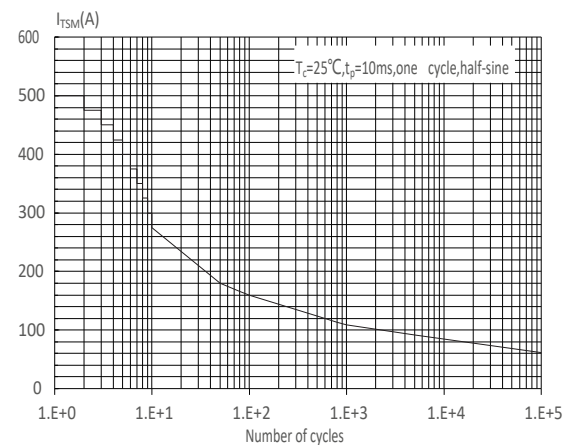
FIG : Non-repetitive surge peak on-state current for a sinusoidal pulse with width t_p < 10ms , and corresponding value of I^2t ( di/dt < 150A/μs )
