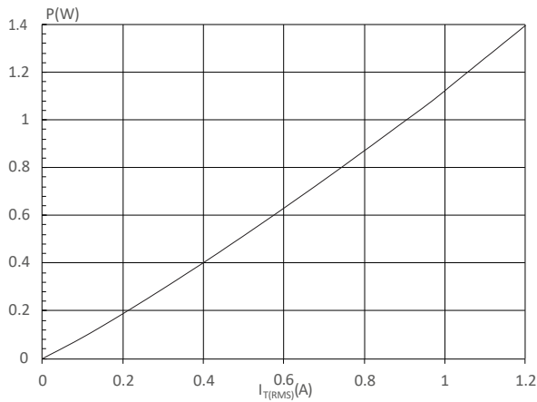
FIG : Maximum power dissipation versus RMS on-state current
