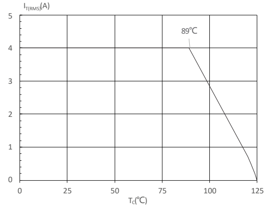
FIG : RMS on-state current versus case temperature
