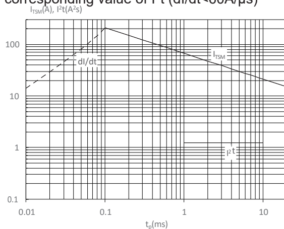
FIG : Non-repetitive surge peak on-state current for a sinusoidal pulse with width t_p < 20ms , and corresponding value of I^2t ( dl/dt < 60A/\mu s )
