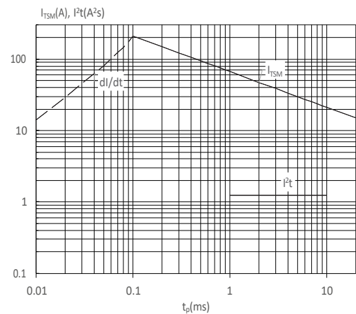
FIG : Non-repetitive surge peak on-state current for a sinusoidal pulse with width t_p < 20\text{ms} , and corresponding value of I^2t ( di/dt < 60\text{A}/\mu\text{s} )
