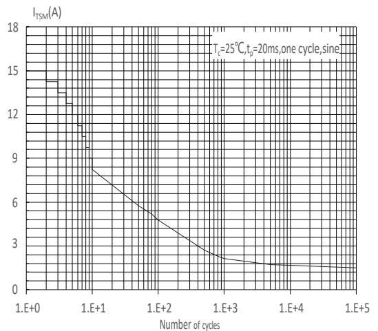
FIG : Non-repetitive surge peak on-state current for a sinusoidal pulse with width t_p < 20ms , and corresponding value of I^2t ( di/dt < 60A/μs )
