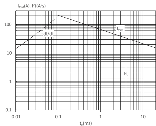
FIG : Non-repetitive surge peak on-state current for a sinusoidal pulse with width t_p < 20ms , and corresponding value of I^2t ( di/dt < 60A/μs )
