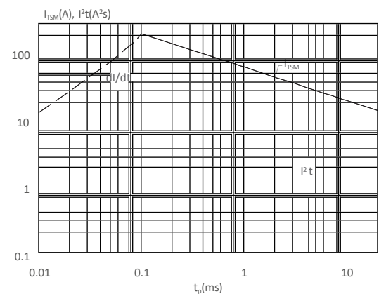
FIG : Non-repetitive surge peak on-state current for a sinusoidal pulse with width t_p < 20ms , and corresponding value of I^2t ( di/dt < 60A/\mu s )
