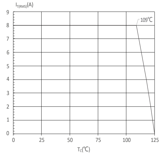
FIG : On-state characteristics
