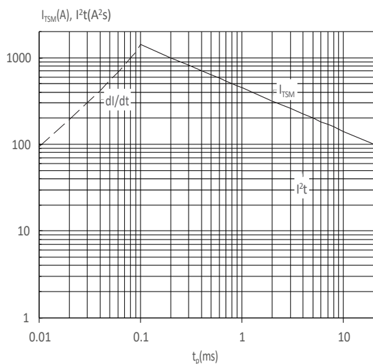
FIG : Non-repetitive surge peak on-state current for a sinusoidal pulse with width t_p < 20ms , and corresponding value of I^2t ( di/dt < 100A/\mu s )
