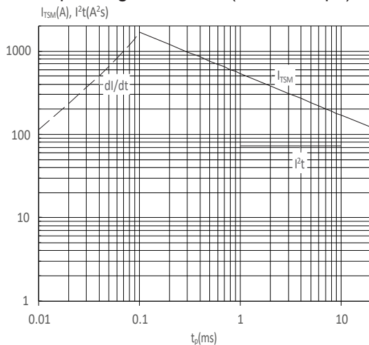
FIG : Non-repetitive surge peak on-state current for a sinusoidal pulse with width t_p < 20ms , and corresponding value of I^2t ( dl/dt < 50A/\mu s )
