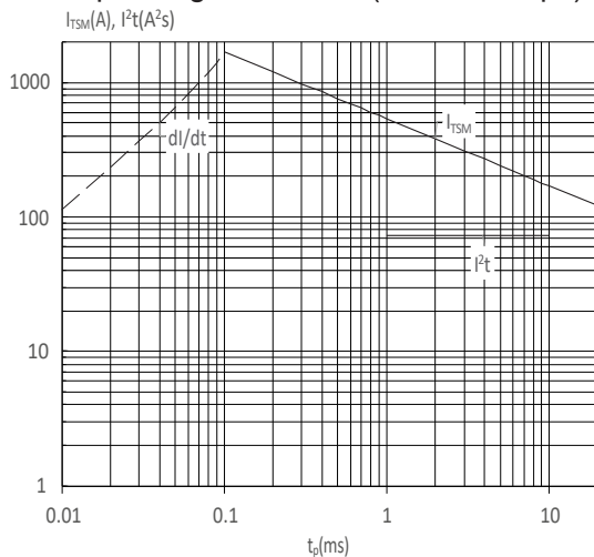
FIG : Non-repetitive surge peak on-state current for a sinusoidal pulse with width t_p < 20ms , and corresponding value of I^2t ( dl/dt < 100A/\mu s )
