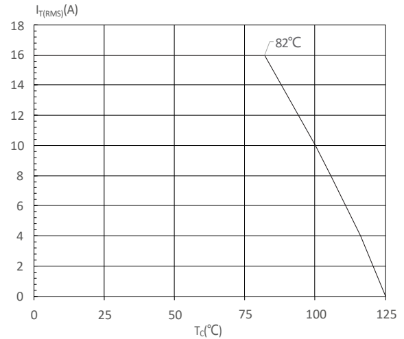
FIG : On-state characteristics
