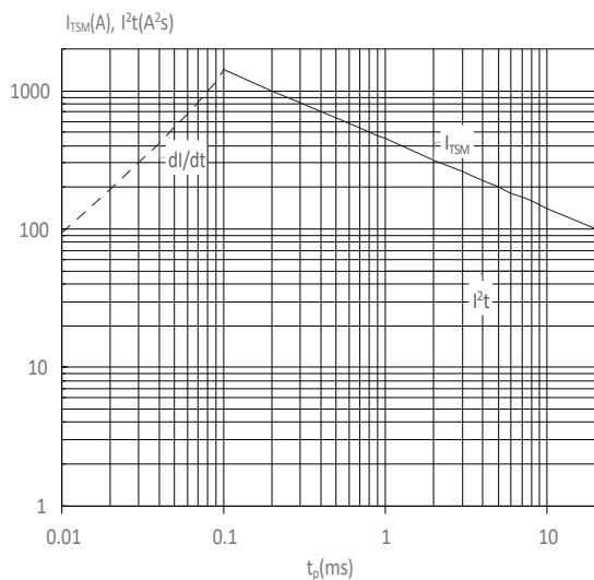
FIG : Non-repetitive surge peak on-state current for a sinusoidal pulse with width t_p < 20\text{ms} , and corresponding value of I^2t ( di/dt < 100\text{A}/\mu\text{s} )
