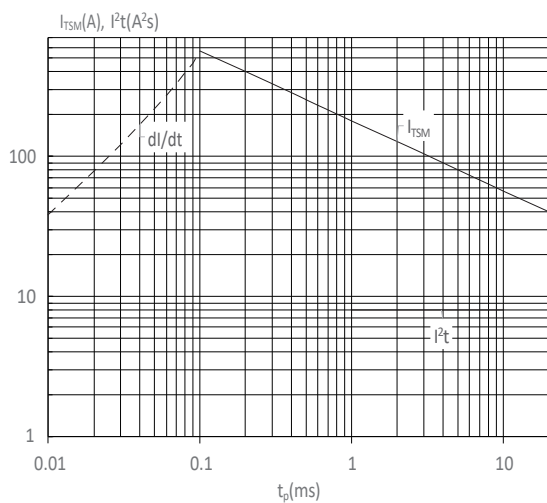
FIG : Non-repetitive surge peak on-state current for a sinusoidal pulse with width t_p < 20\text{ms} , and corresponding value of I^2t ( di/dt < 50\text{A}/\mu\text{s} )
