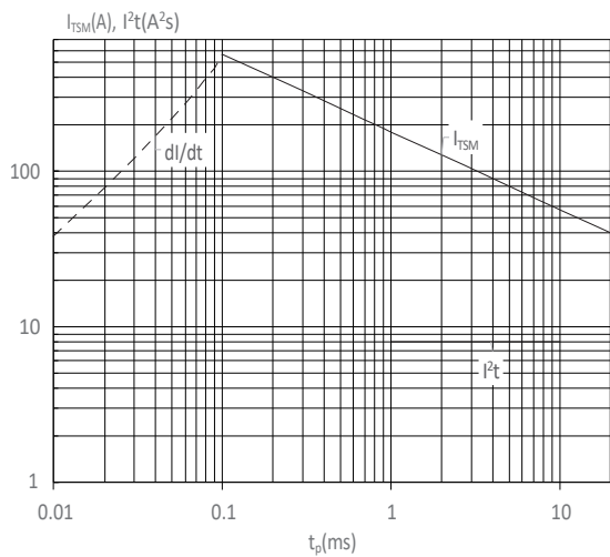
FIG : Non-repetitive surge peak on-state current for a sinusoidal pulse with width t_p < 20ms , and corresponding value of I^2t ( di/dt < 50A/\mu s )
