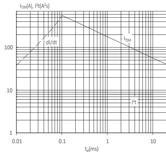
FIG : Non-repetitive surge peak on-state current for a sinusoidal pulse with width t_p < 20ms , and corresponding value of I^2t ( dl/dt < 50A/\mu s )
