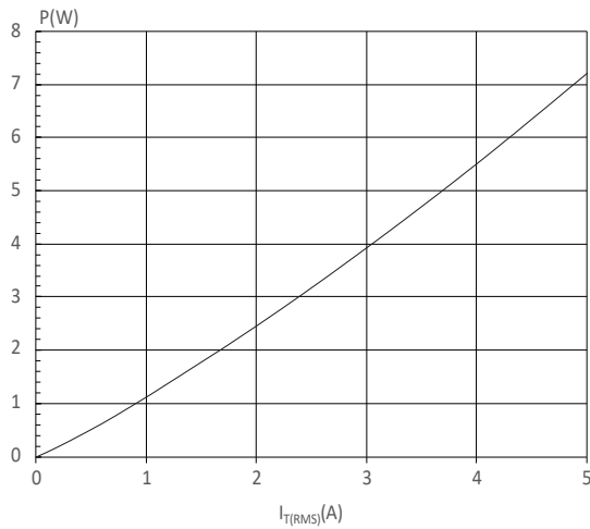
FIG : Maximum power dissipation versus RMS on-state current
