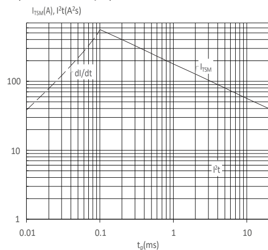
FIG : Non-repetitive surge peak on-state current for a sinusoidal pulse with width t_p < 20ms , and corresponding value of I^2t ( dI/dt < 100A/μs )
