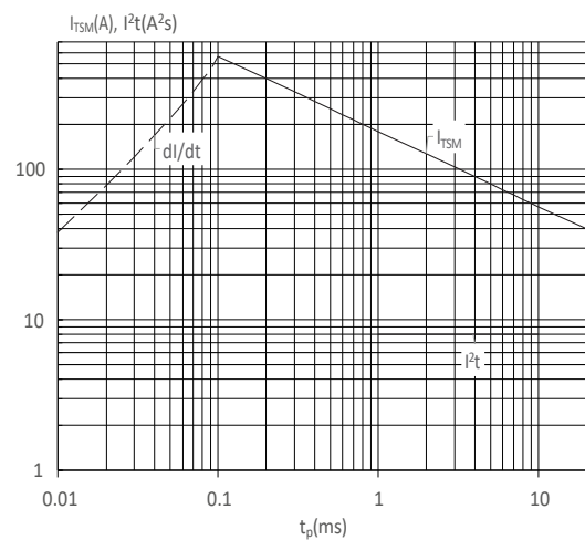
FIG : Non-repetitive surge peak on-state current for a sinusoidal pulse with width t_p < 20ms , and corresponding value of I^2t ( dl/dt < 50A/μs )
