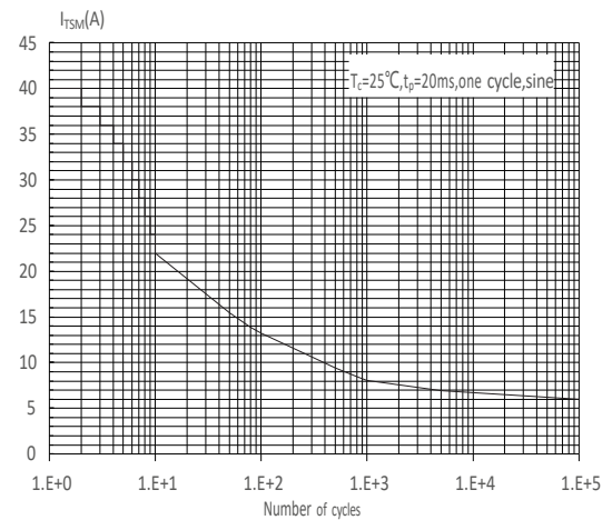
FIG : Non-repetitive surge peak on-state current for a sinusoidal pulse with width t_p < 20ms , and corresponding value of I^2t ( dl/dt < 50A/μs )
