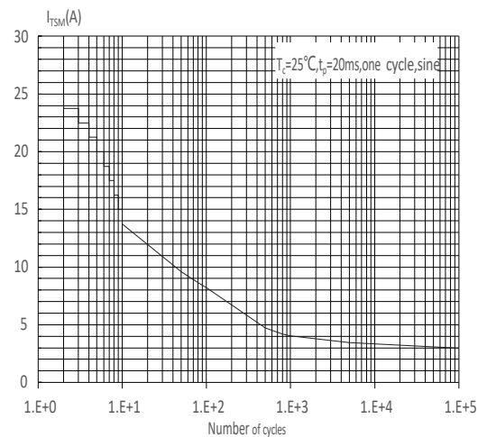
FIG : Non-repetitive surge peak on-state current for a sinusoidal pulse with width t_p < 20ms , and corresponding value of I^2t ( di/dt < 100A/μs )
