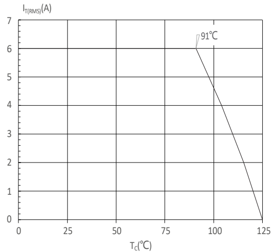
FIG : RMS on-state current versus case temperature
