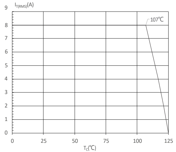
FIG : RMS on-state current versus case temperature
