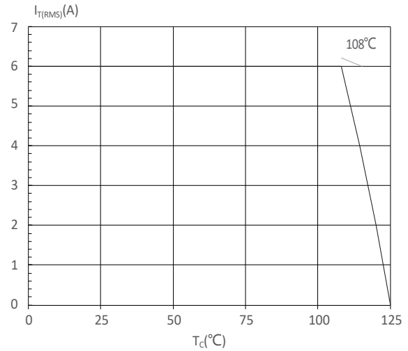
FIG : RMS on-state current versus case temperature
