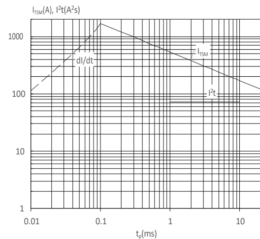
FIG : Non-repetitive surge peak on-state current for a sinusoidal pulse with width t_p < 20ms , and corresponding value of I^2t ( di/dt < 50A/μs )
