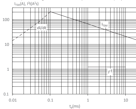
FIG : Non-repetitive surge peak on-state current for a sinusoidal pulse with width t_p < 20ms , and corresponding value of I^2t ( dl/dt < 50A/\mu s )
