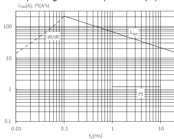
FIG : Non-repetitive surge peak on-state current for a sinusoidal pulse with width t_p < 20ms , and corresponding value of I^2t ( dl/dt < 50A/\mu s )
