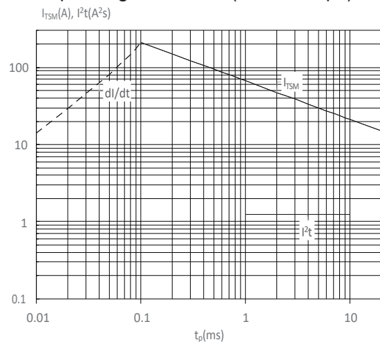
FIG : Non-repetitive surge peak on-state current for a sinusoidal pulse with width t_p < 20\text{ms} , and corresponding value of I^2t ( di/dt < 60\text{A}/\mu\text{s} )
