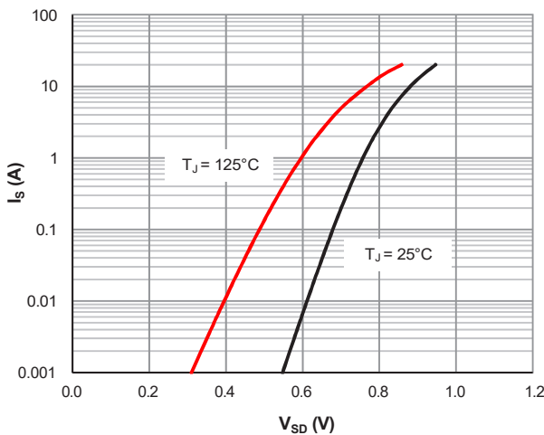
Figure 7: Body-Diode Characteristics
