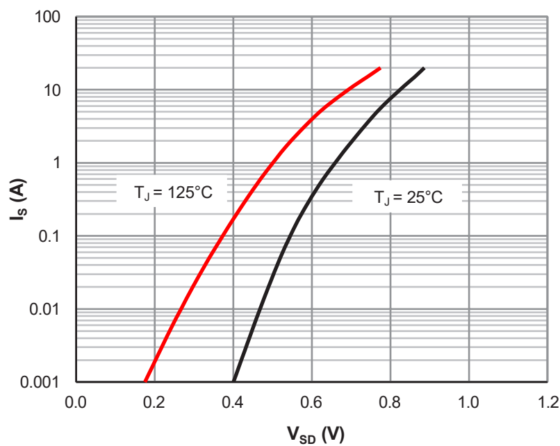
Figure 5: Body-Diode Characteristics
