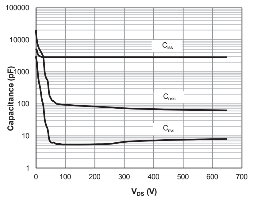
Figure 6: Capacitance Characteristics
