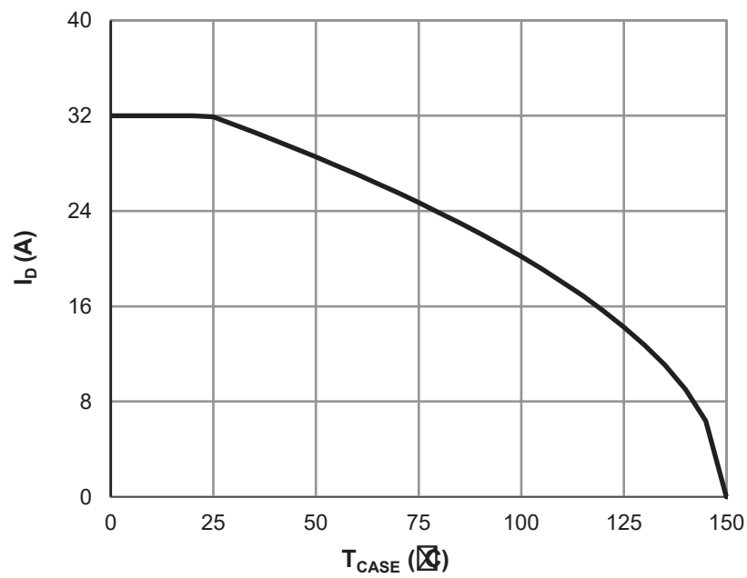
Figure 7: Current De-rating
