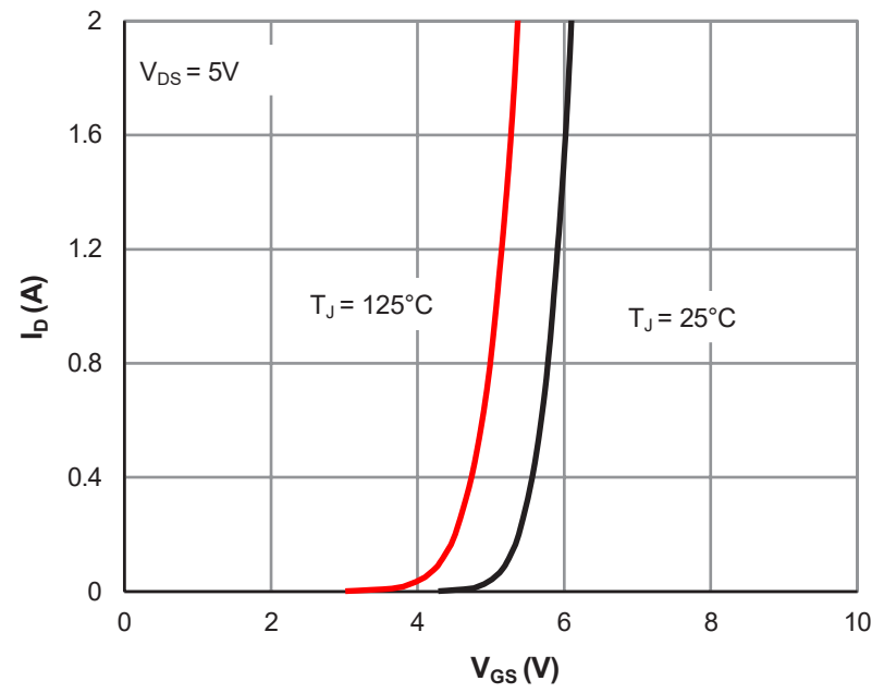
Figure 2: Transfer Characteristics
