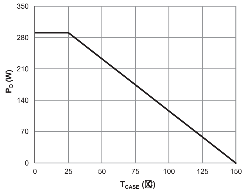
Figure 8: Power De-rating
