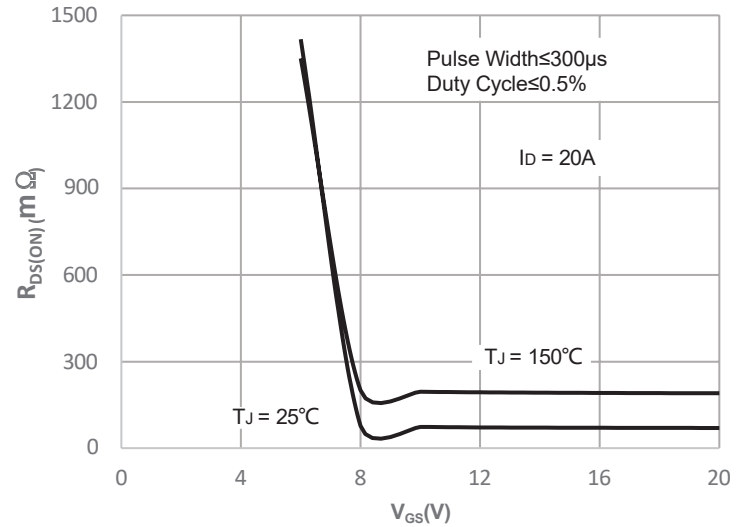
Figure 14: R_{DS(ON)} vs. V_{GS}
