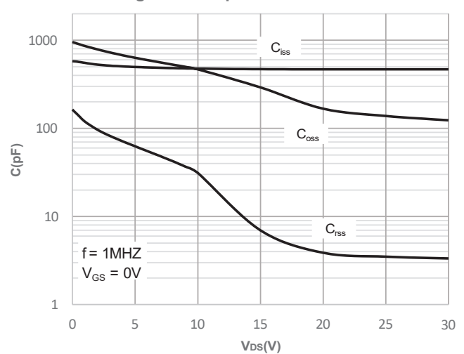
Figure 10: Capacitance Characteristics
