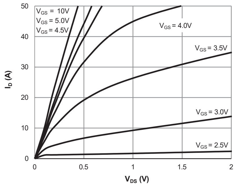
Figure 1: Saturation Characteristics
