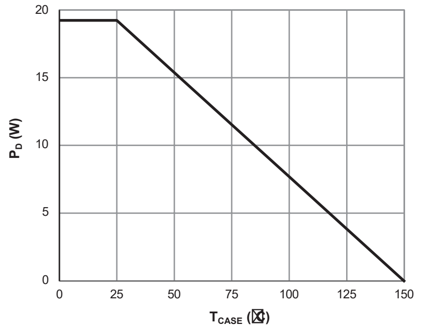
Figure 10: Power De-rating
