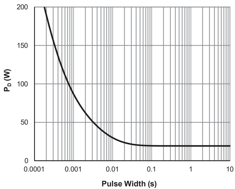
Figure 11: Single Pulse Power Rating, Junction-to-Case
