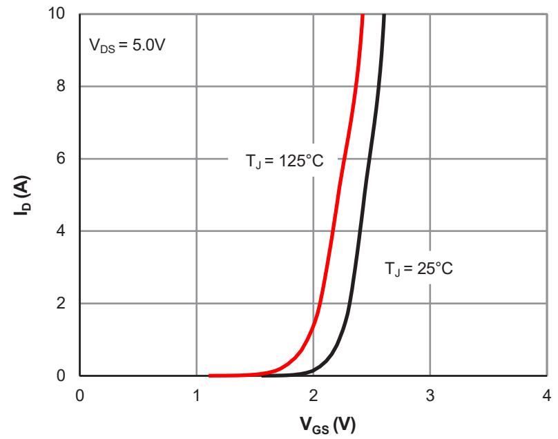
Figure 2: Transfer Characteristics
