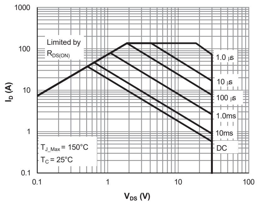
Figure 12: Maximum Safe Operating Area
