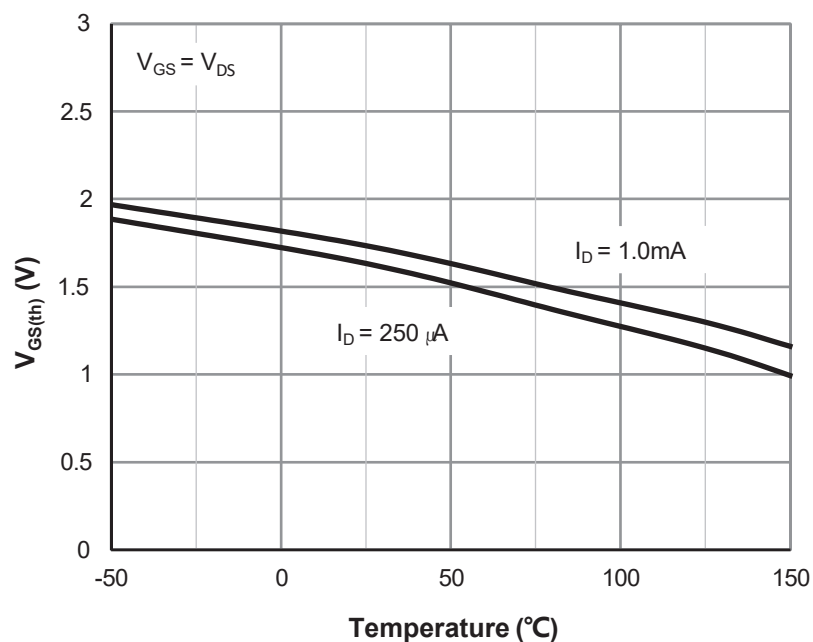
Figure 5: V_{GS(th)} vs. Junction Temperature
