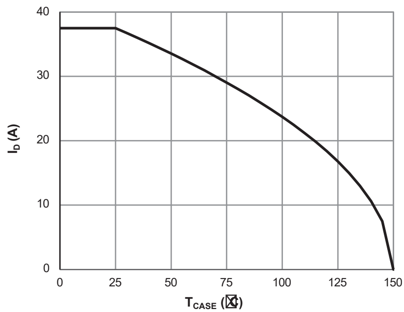
Figure 9: Current De-rating
