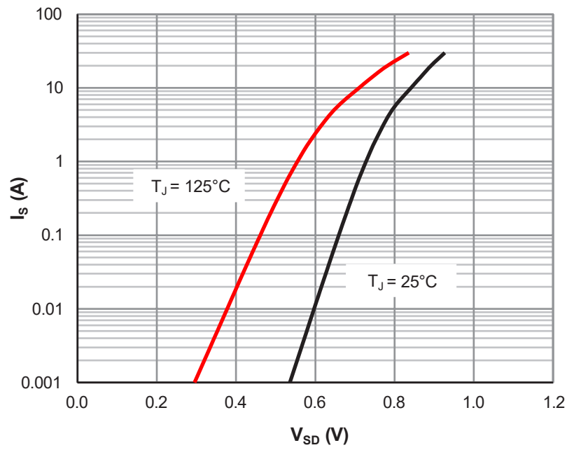
Figure 7: Body-Diode Characteristics
