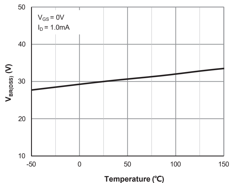
Figure 6: V_{BR(DSS)} vs. Junction Temperature
