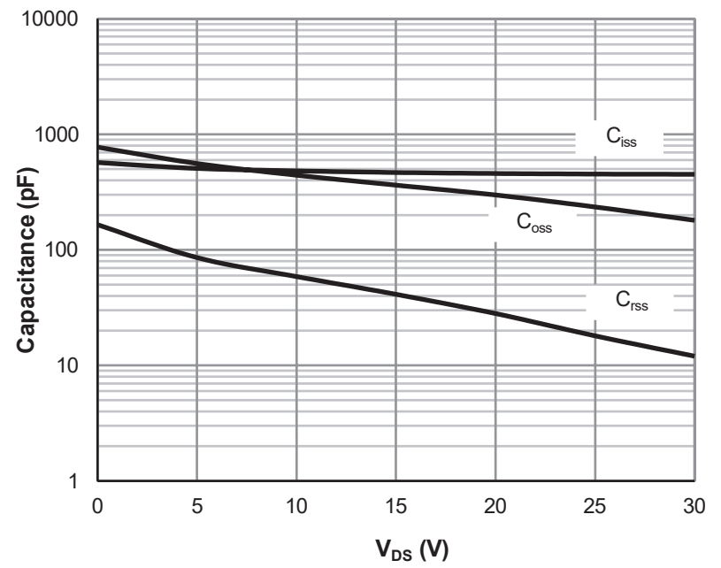
Figure 8: Capacitance Characteristics
