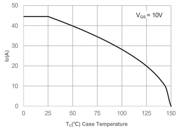
Figure 2: Current De-rating
