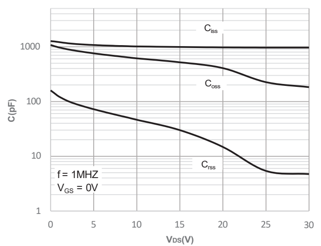
Figure 10: Capacitance Characteristics
