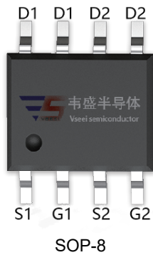
SOP-8
