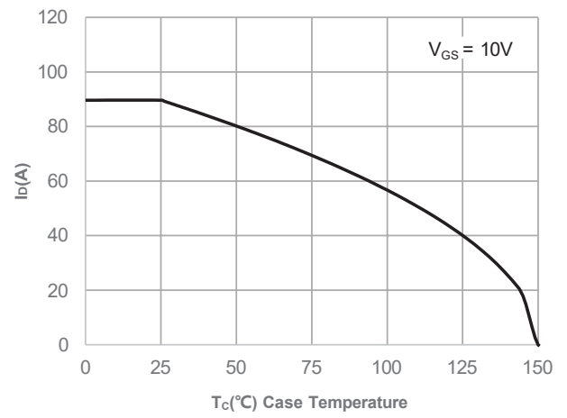
Figure 2: Current De-rating
