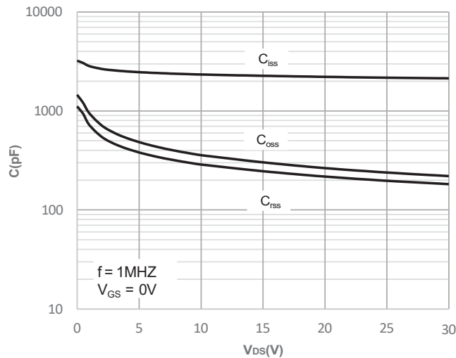
Figure 10: Capacitance Characteristics
