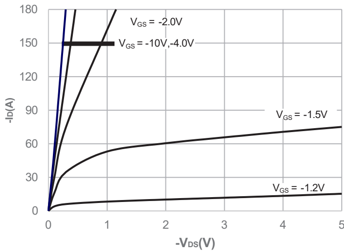
Figure 5: Output Characteristics
