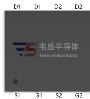
DFN3x3
