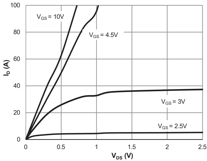
Figure 1: Saturation Characteristics
