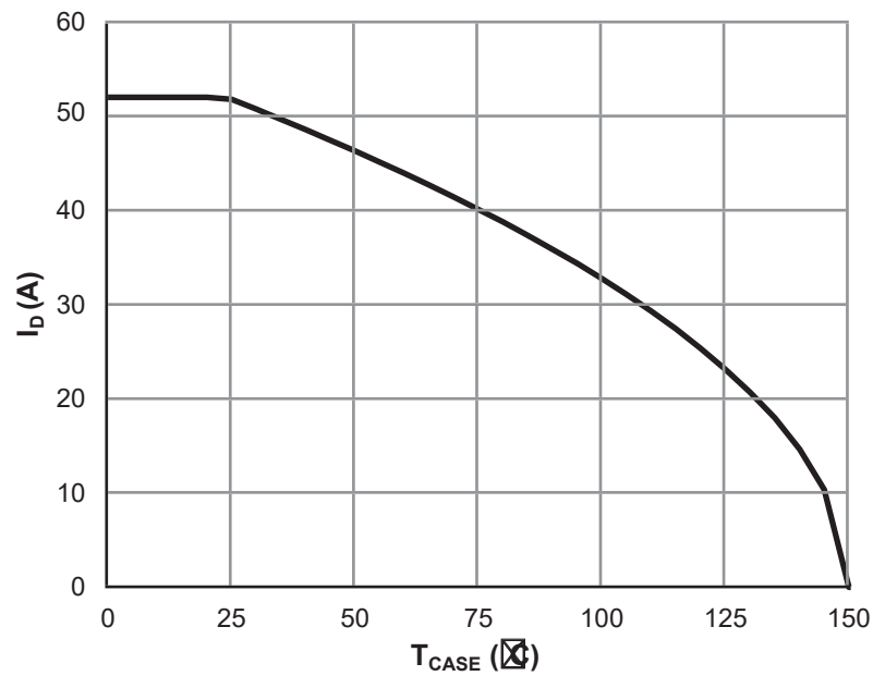
Figure 7: Current De-rating
