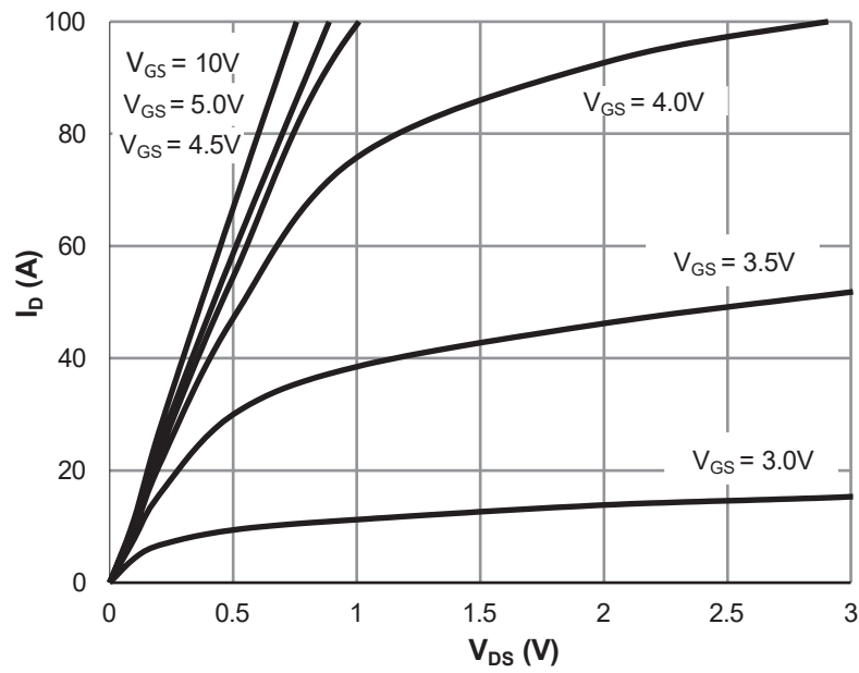
Figure 1: Saturation Characteristics
