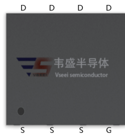
DFN3x3
