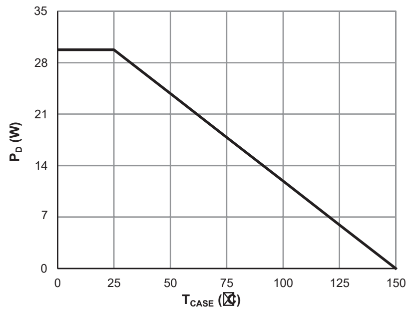
Figure 8: Power De-rating
