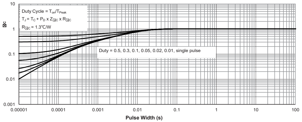
Figure 13: Normalized Transient Thermal Impedance
