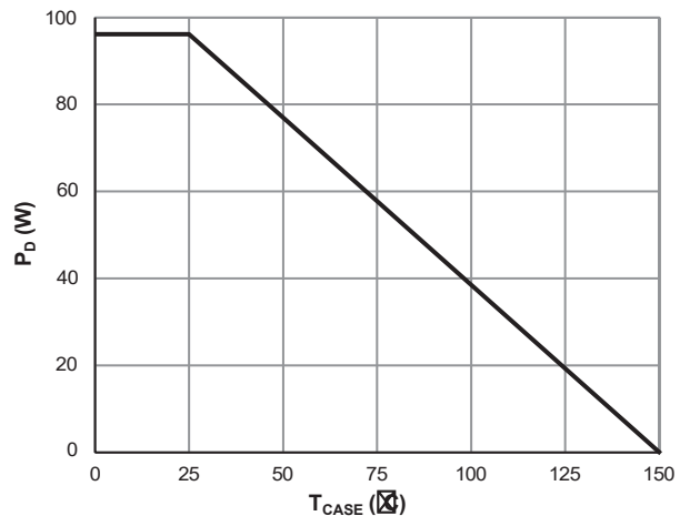
Figure 10: Power De-rating
